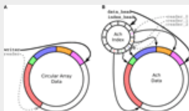
Figure 1. Logical memory structure for a conventional circular buffer (A) and an Ach channel (B). (A) shows a single writer, single reader circular buffer. (B) shows the Ach data structure with separate index and data buffers. The index buffer records metadata on the messages, enabling multiple readers, and detection of overwritten messages.
